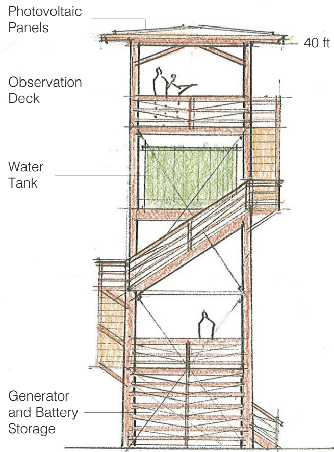
Water Tower South Elevation and Plan GTN Mission, Santo Antônio Amazonas, Brasil
