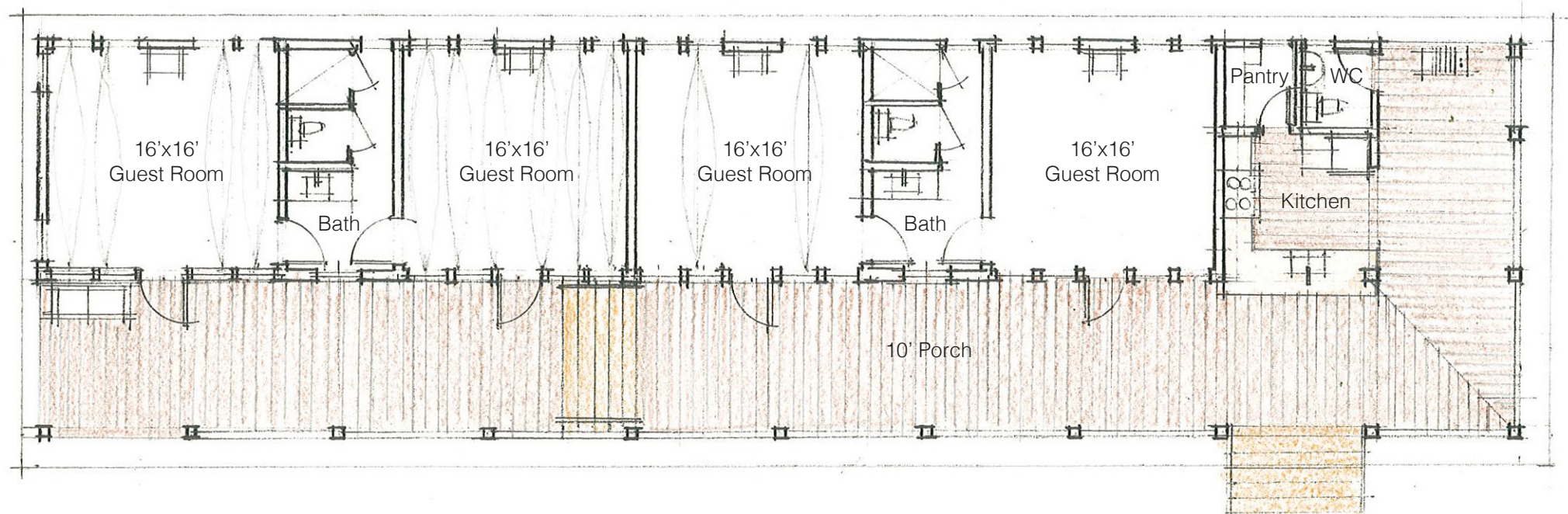
Guest House West Elevation and Floor Plan
